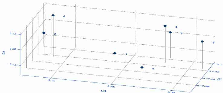
Diagram 4: Correspondence analyses of genetic similarity of Scots pine analyzed populations in three dimensions after Sokal and Michener
